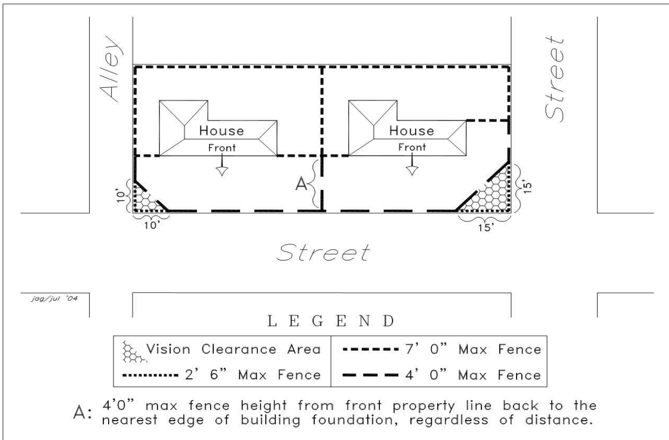
Diagram: Allowed Fence Heights & Vision Clearance Areas
